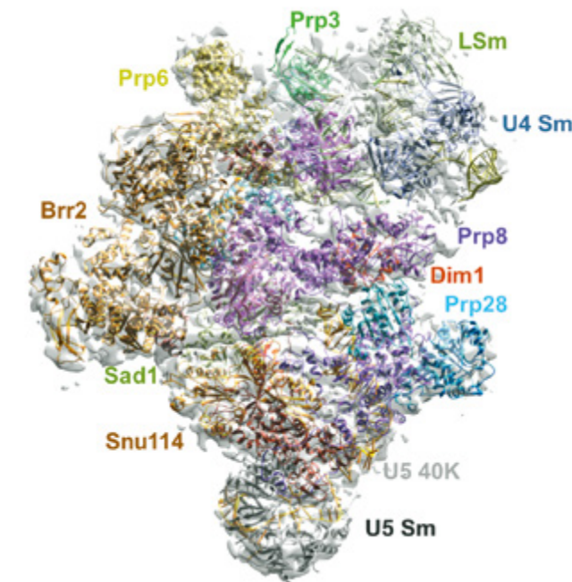
◀ Architecture of the human U4/U6.U5 tri-snRNP, the largest preformed subunit of the spliceosome (cryo-EM structure).
