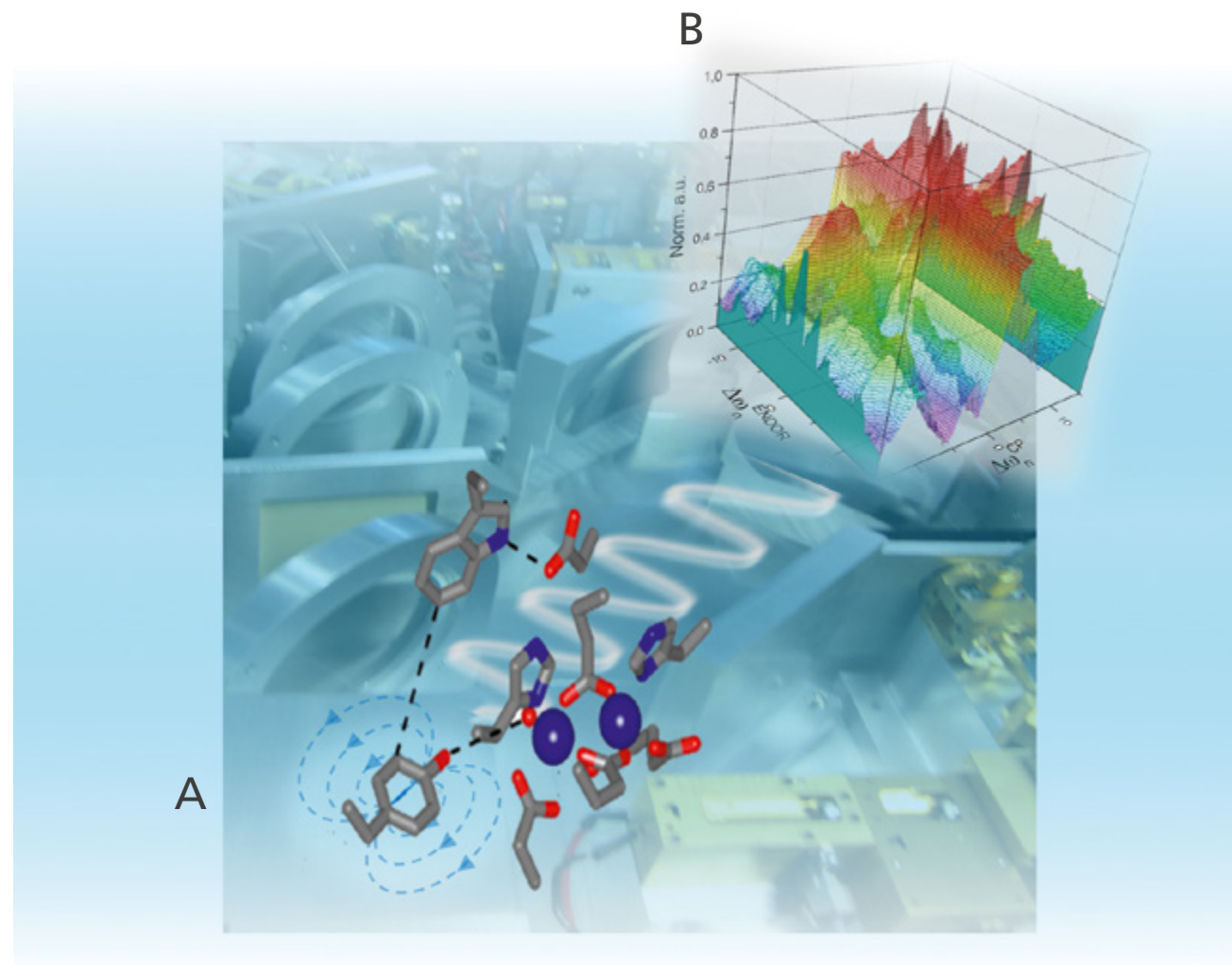
▲ The image shows an EPR experiment to observe the active site of an enzyme. Represented are: A) the structure of a protein radical in E. coli RNR with surrounding amino acids and B) a high-frequency (94 gigahertz) electron-nuclear double resonance (ENDOR)-spectrum of protons that are in the vicinity of this radical. Background: View of the microwave bridge for EPR in quasi-optical regime.
