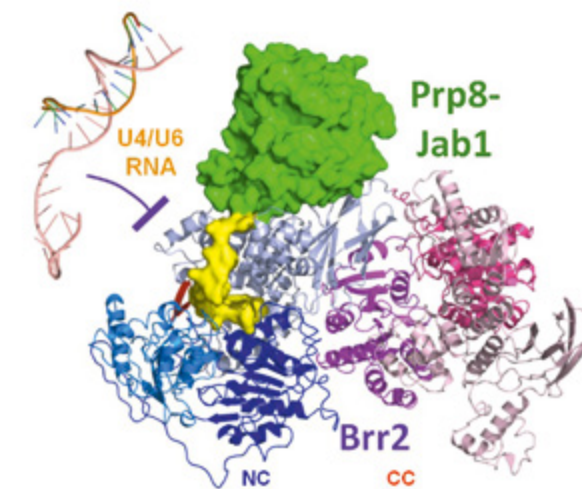
▲ The enzyme Brr2 plays a key role during the catalytic activation of the spliceosome and is regulated by Prp8's Jab1 domain (X-ray crystal structure of the Brr2-Jab1 complex).
