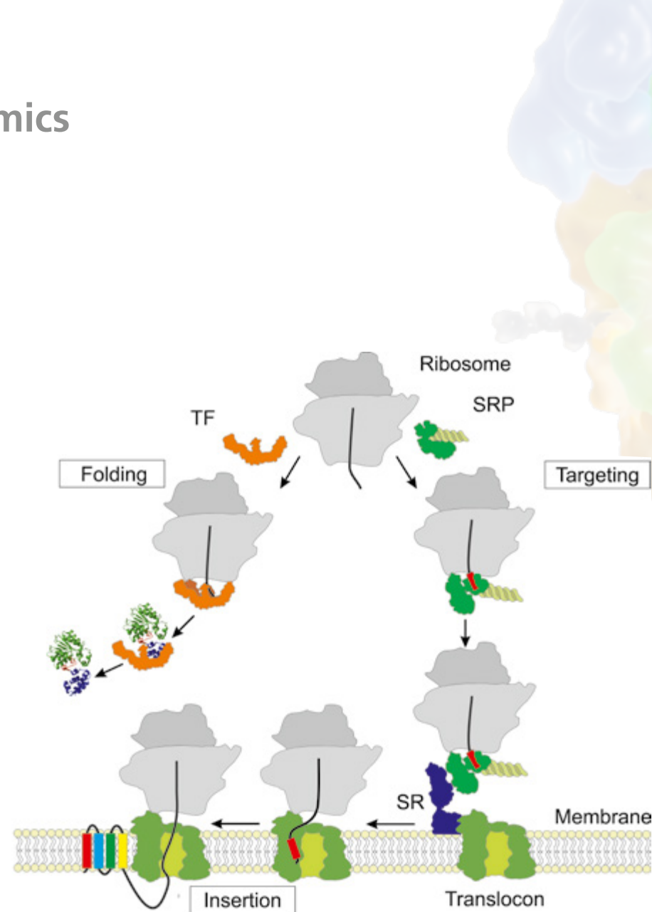
▲ Figure 1: Interaction of protein biogenesis factors with the nascent peptide chain on the ribosome. The signal sequence, which is recognized by SRP, is highlighted in red.
