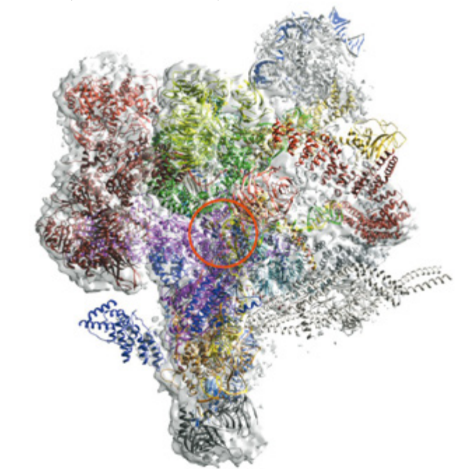
▲ A catalytically active spliceosome has a complex three-dimensional structure. Red circle: position of the catalytic center.
