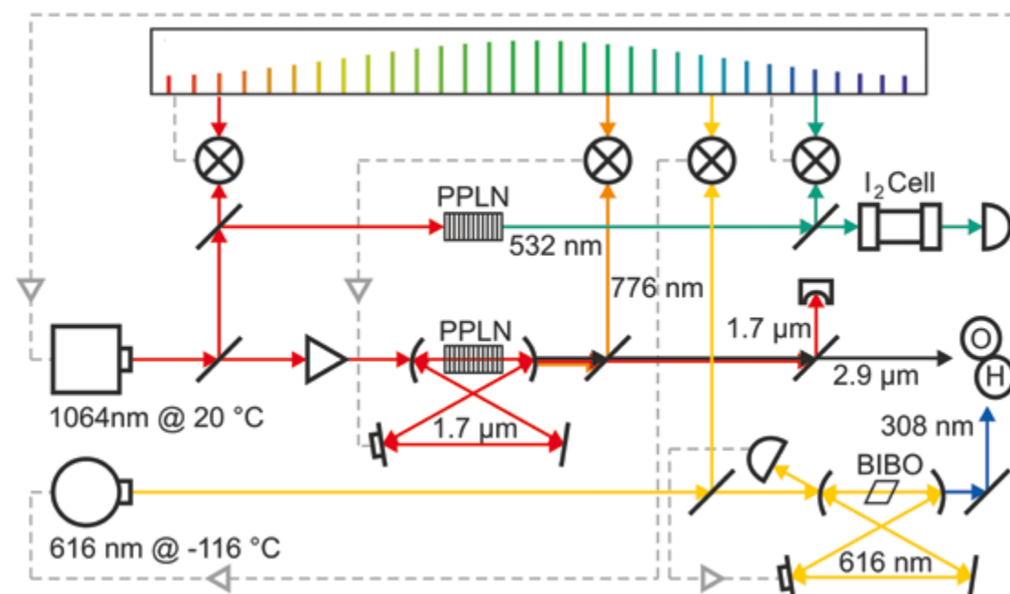
▲ A simplified overview of the laser system for the hydroxyl molecule spectroscopy experiment.
