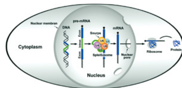
▲ Spliceosomes remove introns from a pre-mRNA to produce mature mRNA which serves as a template for protein production outside the nucleus.
