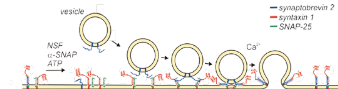
◀ The fusion of membranes is mediated by SNARE proteins (blue, red, and green).
