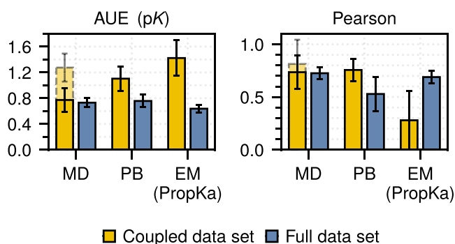
Figure 3. Performance of methods on coupled residues. Average unsigned errors (AUEs) and Pearson correlation coefficients were computed for both the coupled data set (i.e., 18 aspartates and glutamates) and the full data set aspartate and glutamate residues, with the coupled set discarded. Dashed lines indicate the performance of the MD-based approach before coupling was accounted for (see text). Bootstrapped standard errors are depicted.
